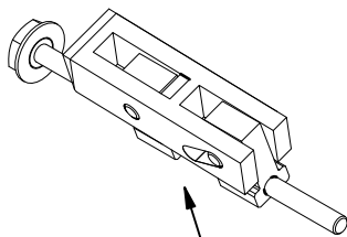
ENDCLAMP
