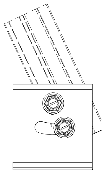
TILT LEG RAIL ON SWIVEL L-PLATE
