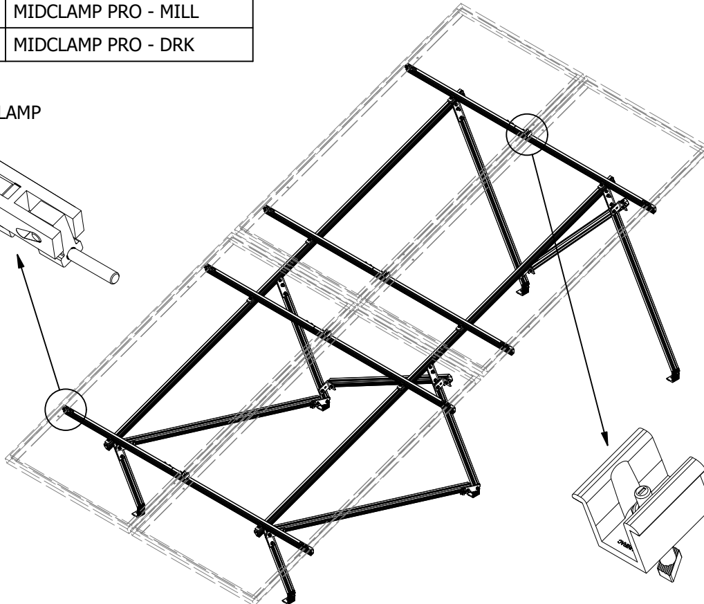
MIDCLAMP
